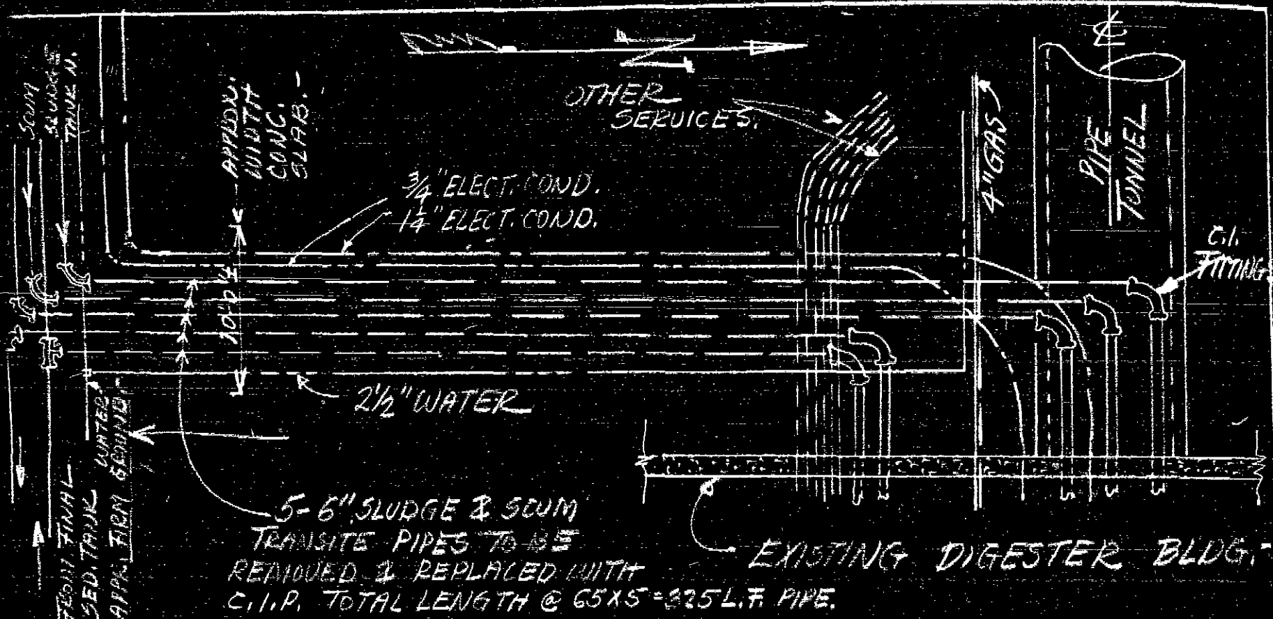
PLAN OF SLUDGE PIPING SCALE \frac{1}{8}" = 1 \text{ FOOT.}
